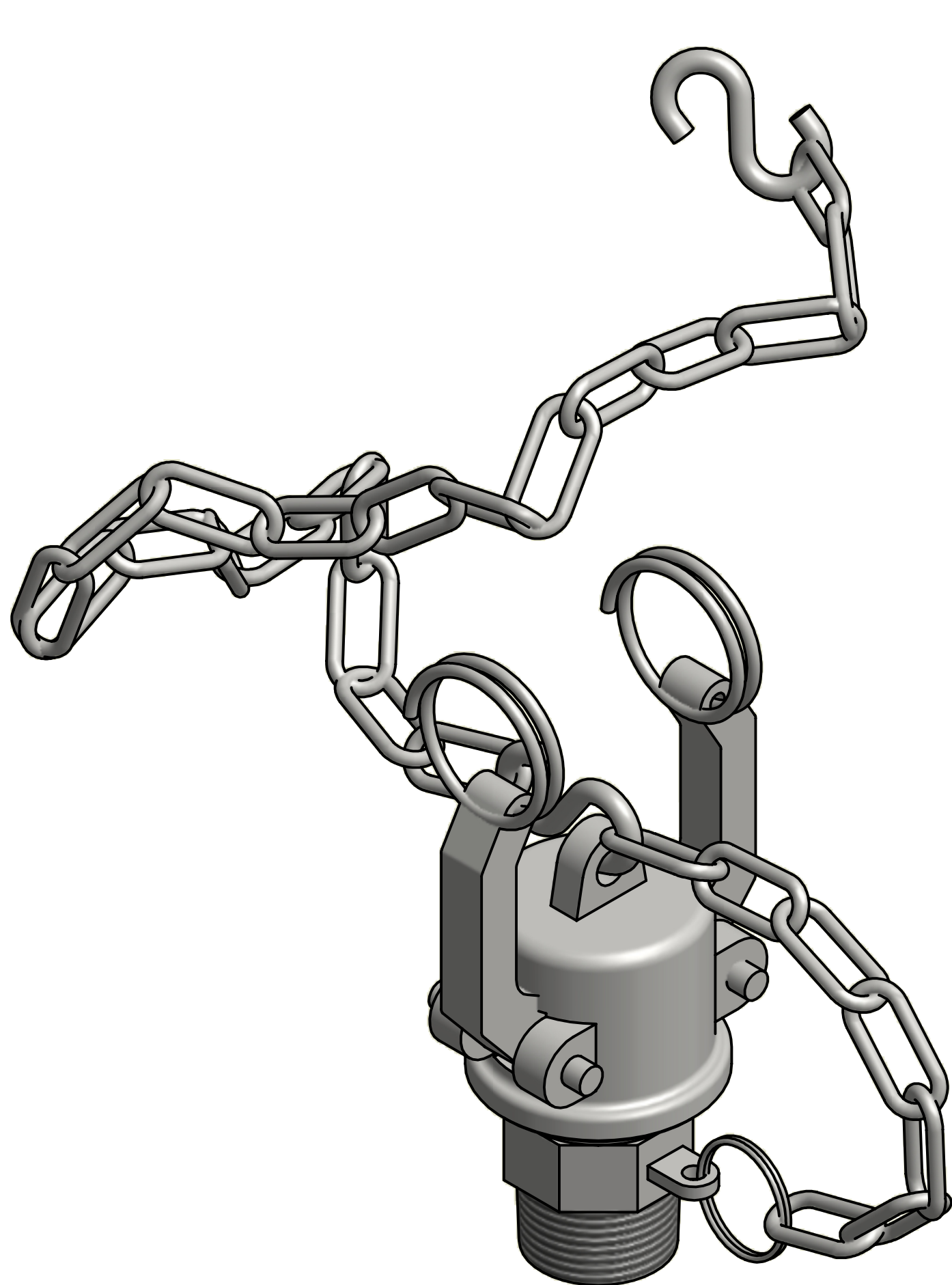
ISOMETRIC VIEW
